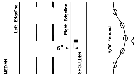
FREEWAYS AND EXPRESSWAYS
