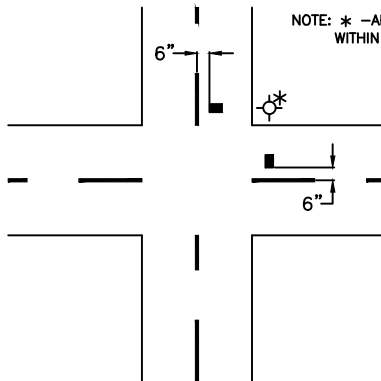
TWO LANE STREET AT INTERSECTION
