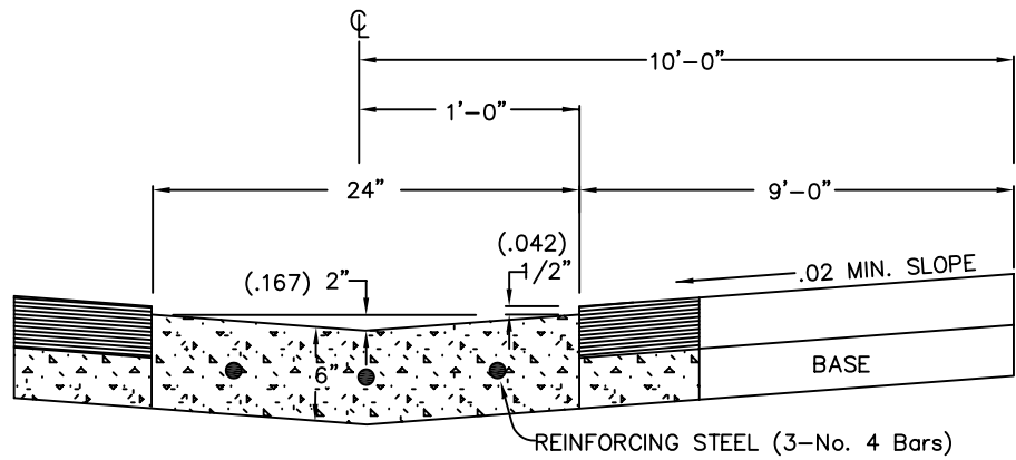
GUTTER DETAIL
