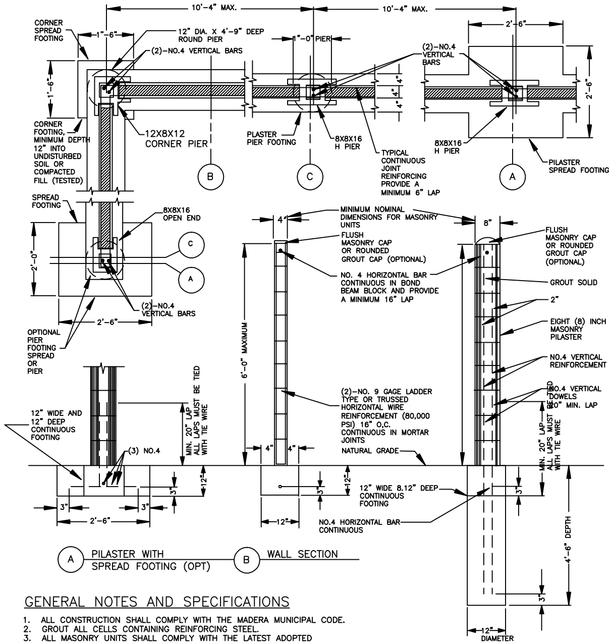
C PILASTER WITH PIER FOOTING
